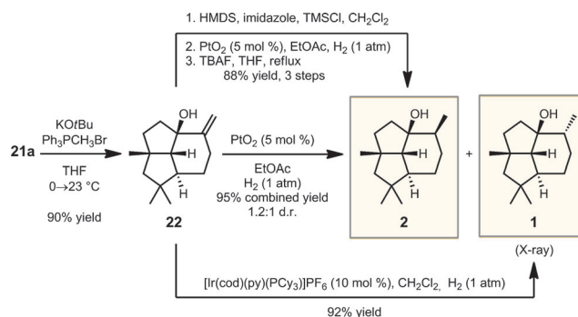
Scheme 3. Synthesis of the reported structures of 9- epi -presilphiperfolan-1-ol ( 2 ) and presilphiperfolan-1-ol ( 1 ).
