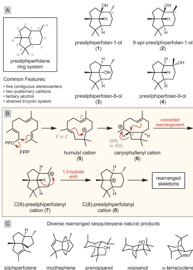
Figure 1. Presilphiperfolanyl (prebotrydial) cations as key intermediates in the biosynthesis of diverse sesquiterpenes.
