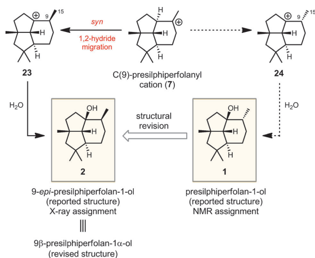
Figure 3. Biosynthetic proposal for the formation of 2 , and structural revision of 1 .
