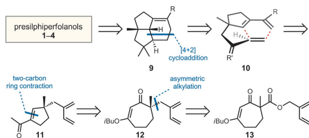
Figure 2. Synthetic strategy toward the presilphiperfolane core.
