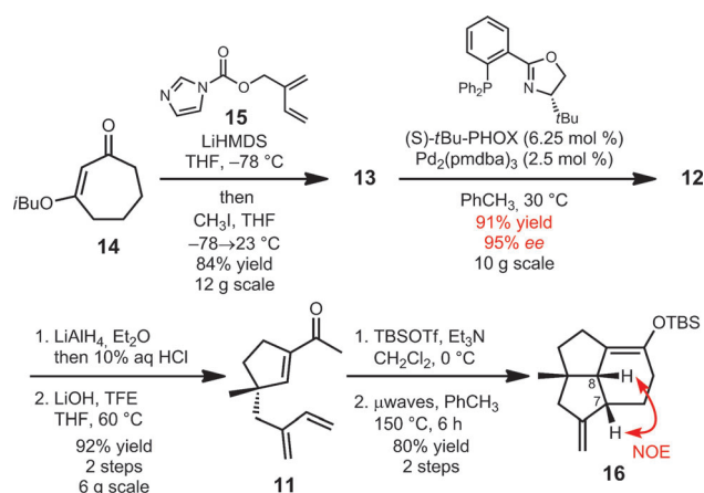
Scheme 1. Gram-scale synthesis of acylcyclopentene 11 and IMDA. HMDS = hexamethyldisilazane, pmdba = 4,4'-methoxydibenzylideneacetone, TFE = 2,2,2-trifluoroethanol, TBS = tert -butyl dimethylsilyl, NOE = nuclear Overhauser effect.
